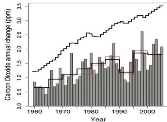
Figure 23: The year-to-year increase of CO 2 vs. time. The bar graph shows an increase in the atmospheric levels, an irregular pattern that correlates well with El Niño warming events and volcanic cooling events. Yet the release of CO 2 from fossil-fuel burning (upper curve) increases smoothly [IPCC 2007, p. 516]. Presumably, there are strong temperature-dependent variations in the CO 2 absorption of the ocean.
