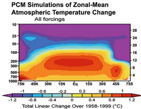
Figure 7: Greenhouse-model-predicted temperature trends versus latitude and altitude; this is figure 1.3F from CCSP 2006, p. 25, and also appears in Figure 6 of the current report. Note the increased temperature trends in the tropical mid-troposphere, in agreement also with the IPCC result [IPCC-AR4 2007, p. 675].
